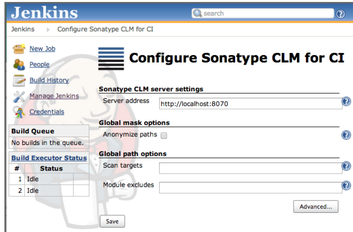
Figure 2.2: Global Configuration of Sonatype CLM for CI in Jenkins
